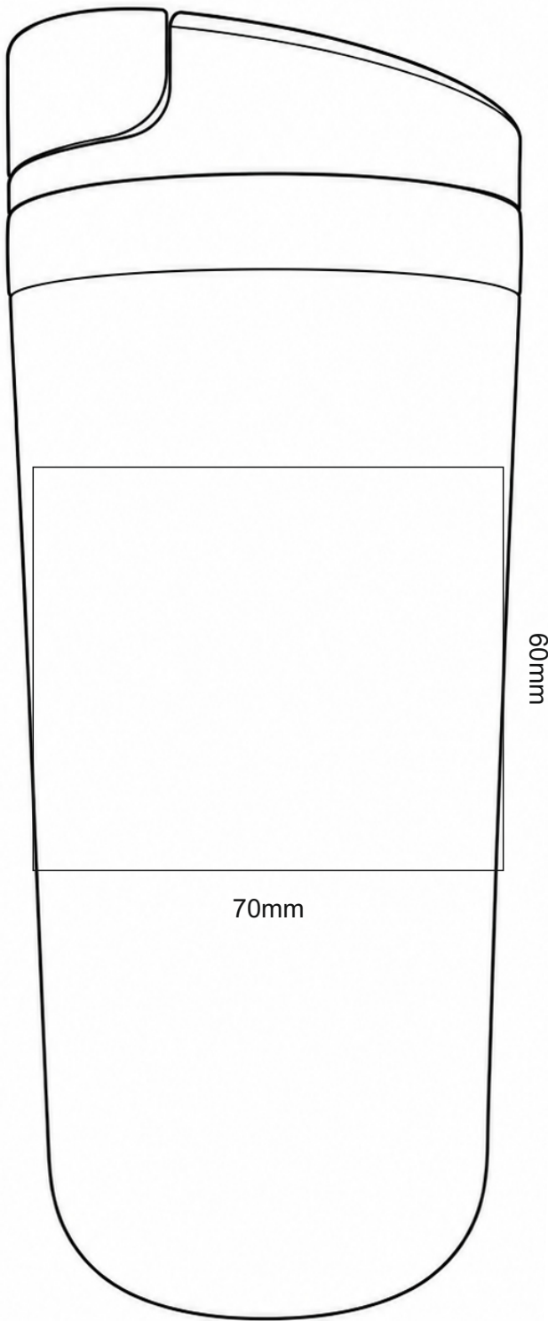
Rotary Engraving
