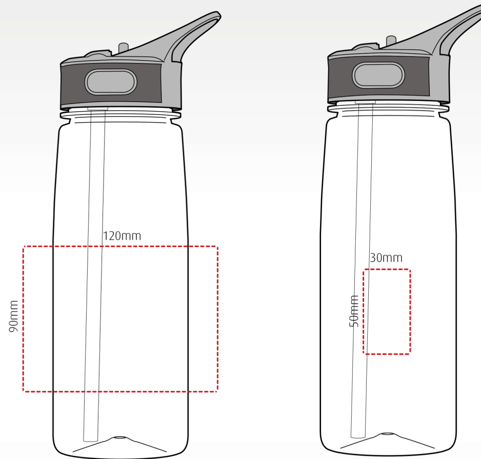
2-3 spot colours pad print
